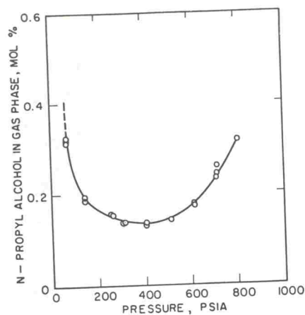
Figure 5. Gas-phase data
